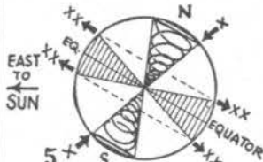
5 EXPANSION WELL UNDER WAY IN THIS POSITION WHICH IS APPROXIMATELY THAT OF THE EARTH.
