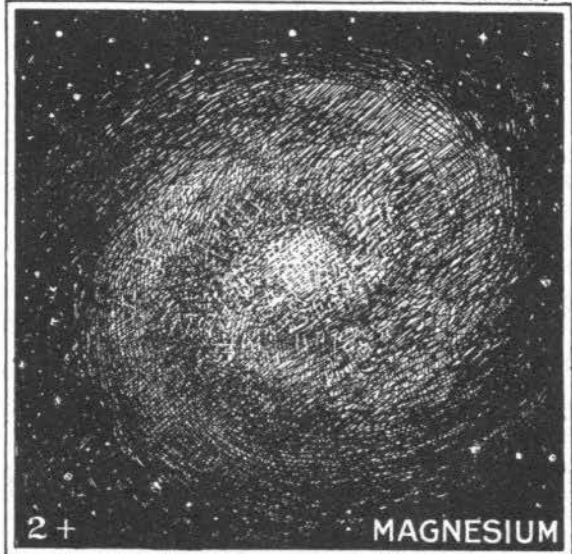
2+ . Electricity gains in second tone. Positive charge is forming a nucleus. Form is ovoid. Expansion of ecliptic narrowing.
