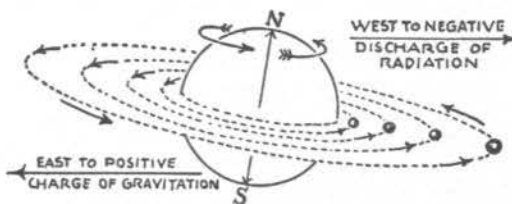
Jupiter is well on the way toward turning its poles upside down. Its rotation is at a considerable inclination to the solar equator though still direct.
