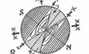
8 THIS IS THE POSITION OF NEPTUNE, OPPOSITE TO THAT AT BIRTH.
