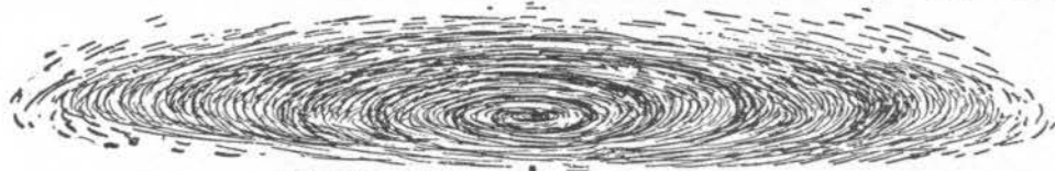
NEBULOUS 1+ PLANE
