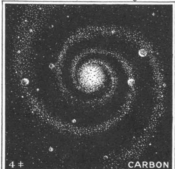
4+ . Maximum positive charge has gathered into definite nucleus and magnetic resistance registered in heat.
