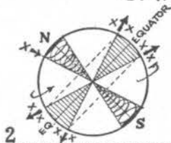
2 MAGNETIC BASES CONTRACT TOWARD POLE AND ECLIPTIC CONTRACTS TOWARD PLANE OF EQUATOR.
