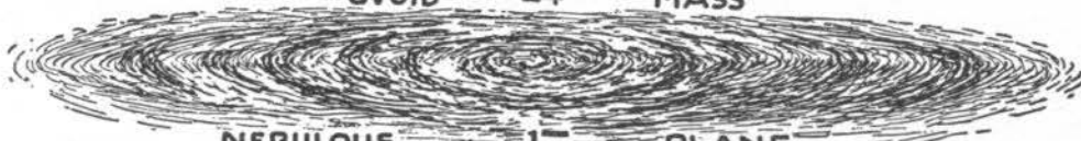
NEBULOUS 1- PLANE
