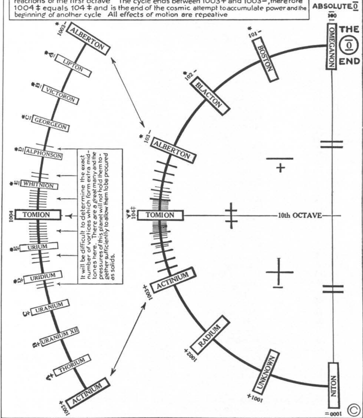
TENTH OCTAVE CONSTANT WHERE TIME DIMENSION OVERTAKES POWER DIMENSION IN PRESSURES WHICH EJECT BETA EMANATIONS AT 186,400 MILES PER SECOND. THIS ENDS THE CYCLE.
