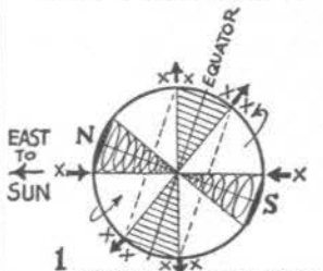
1 IN NEW BORN PLANETS DIMENSIONS OF ECLIPTIC AND MAGNETIC BASES ARE SAME AS PARENT'S.
