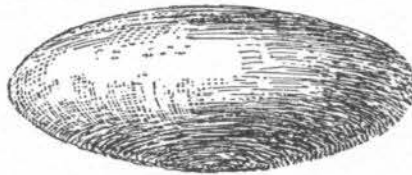
OBLATENESS 3+ DECREASES
