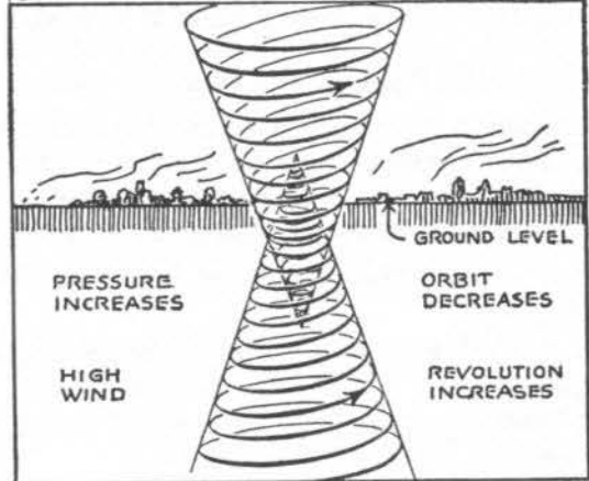
Energy is generated in contracting cones.
