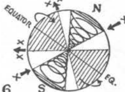
6 MAGNETIC BASES AND ECLIPTIC EXPANDING AND NEARLY MEETING.
