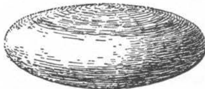
OBLATENESS 3- INCREASES
