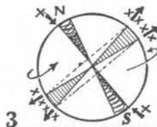
3 MAGNETIC BASES RAPIDLY DISAPPEARING IN POLE & ECLIPTIC REVOLVING IN PLANE
