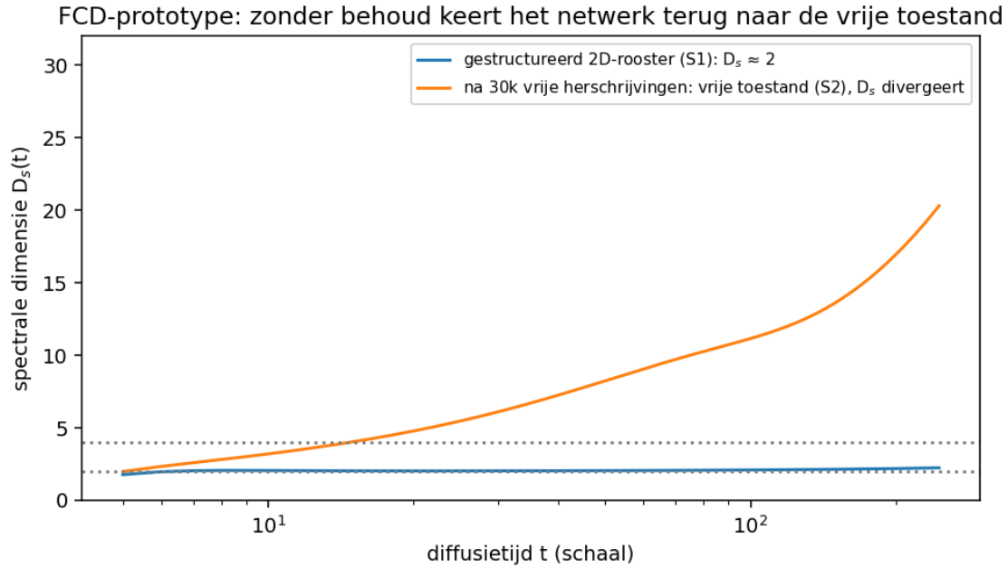
Figure 1. Spectral dimension D_s(t) before and after 30,000 unconstrained local rewrite steps. The initial lattice measures D_s \approx 2 ; the rewritten network has returned to the free, maximally connected state, and its apparent dimension diverges.
