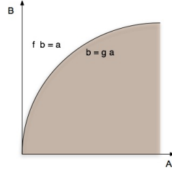
Figure 5.1.: Graphical interpretation of equation (5.136): (a) relation
